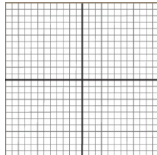
Graph Coordinates
