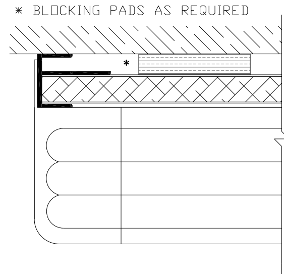
TOP SECTION VIEW SCALE: 1/2
